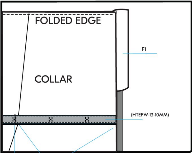
CHINGUARD Inside sketch left side
